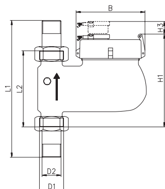
Dimensions MNK-I-N-ST
