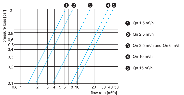
Head loss curves
