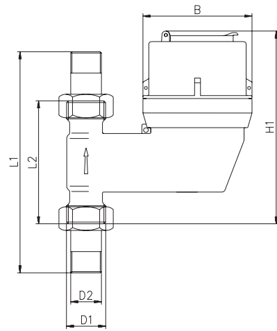
Dimensions Patrol-MNK-ST
