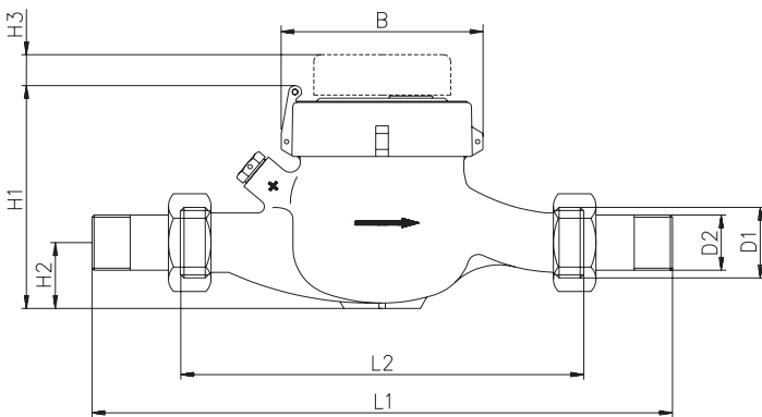
Dimensions MTK-I-N
