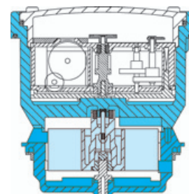
Cross-sectional drawing MNK
