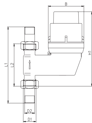
Dimensions Patrol-RTK-ST
