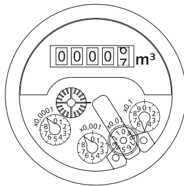
Dial MNK-I-N-ST
