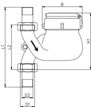
Dimensions MTW-F
